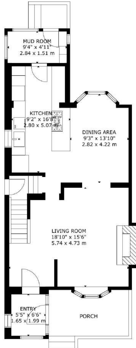
MAIN FLOOR
