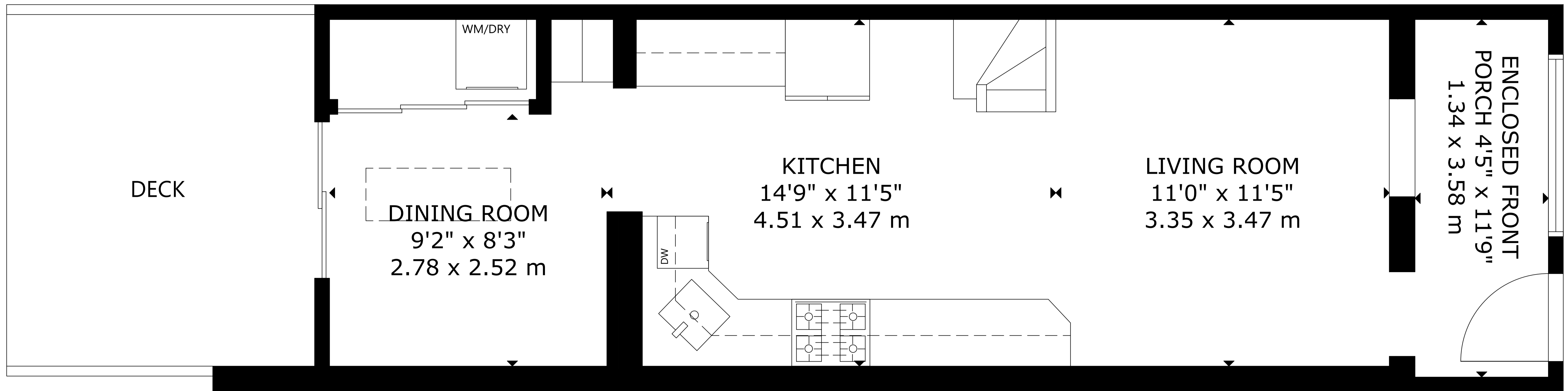
MAIN FLOOR
