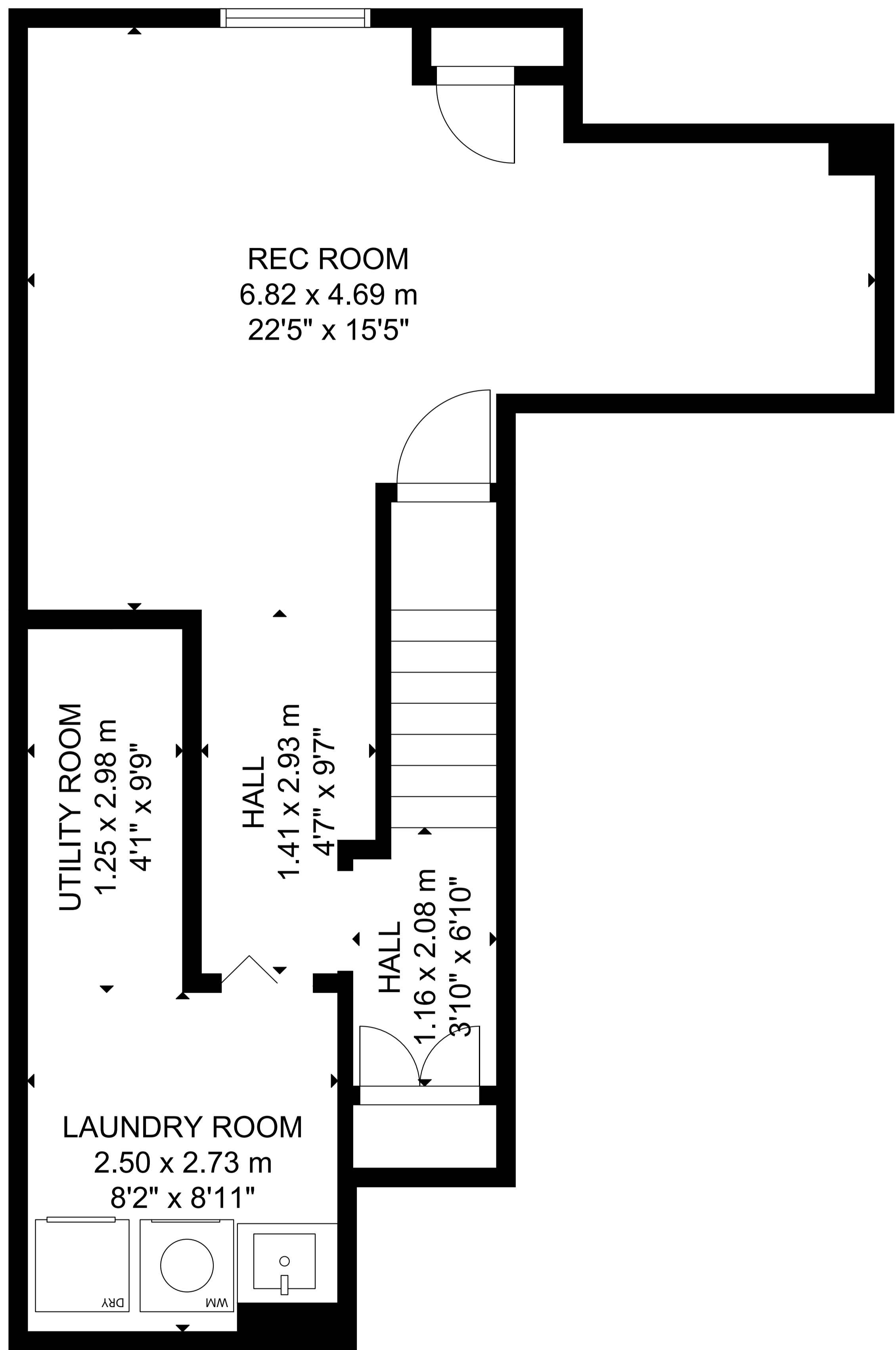
LOWER LEVEL
