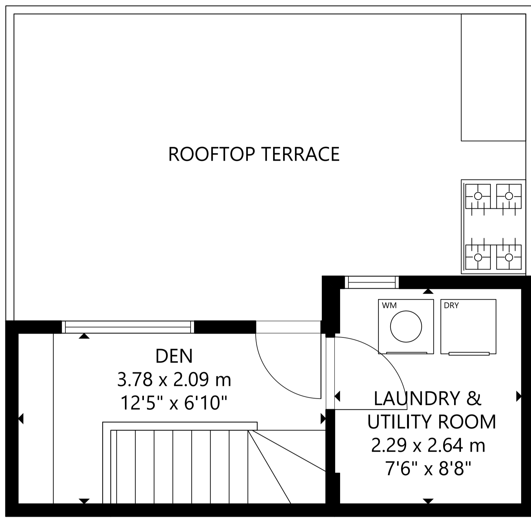
THIRD LEVEL
