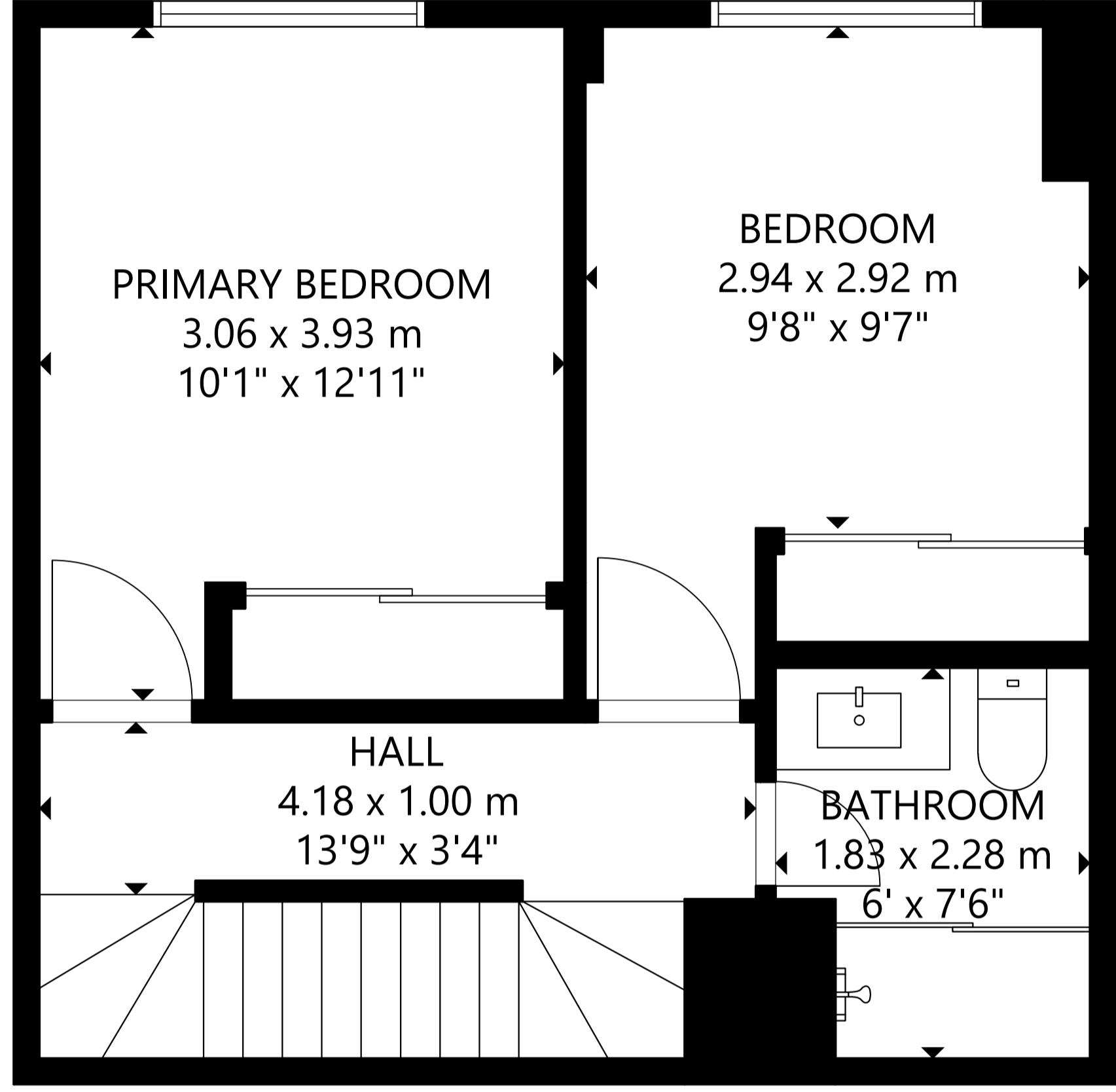
SECOND FLOOR
