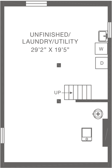
LOWER LEVEL 647 SQUARE FEET
