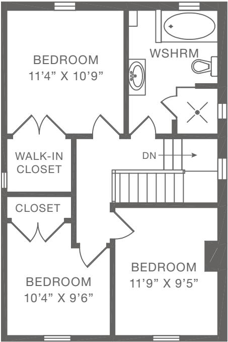
SECOND FLOOR 647 SQUARE FEET
