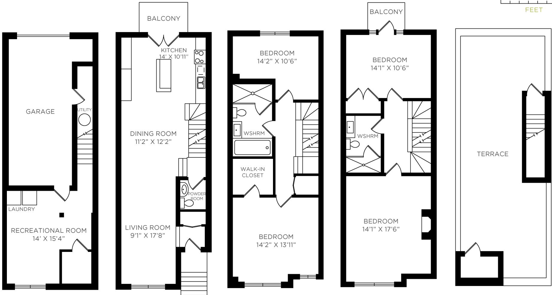
GROUND FLOOR 286 SQUARE FEET
