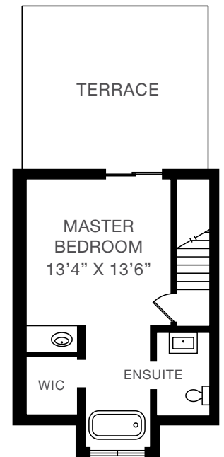
THIRD LEVEL 426 SQUARE FEET
